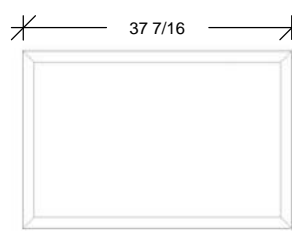
2x 2582 WINDOW
